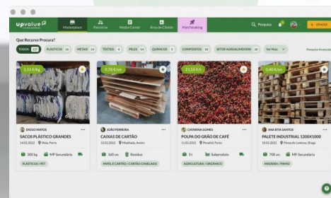
MATCHMAKING ALGORITHM
